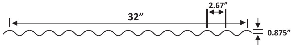
7/8" CORRUGATED
