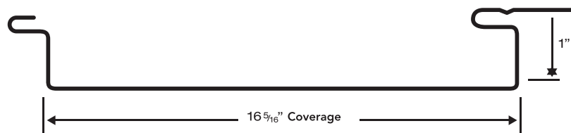
Flat Panel
