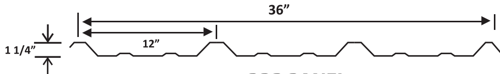
PBR PANEL
