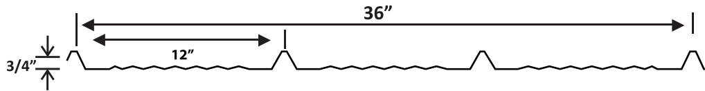
Legacy Panel
